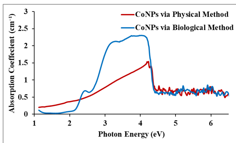
Fig. 7: Absorption coefficient of CoNPs synthesized by physical and biological methods
