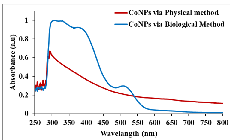
Fig. 6: Absorbance spectra of CoNPs synthesized by physical and biological methods
