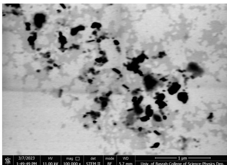
Fig. 4: TEM image of CoNPs synthesized by physical method
