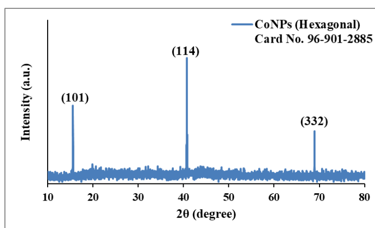
Fig. 3: XRD pattern of CoNPs synthesized by biologically
