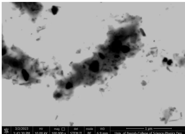
Fig. 5: TEM image of CoNPs synthesized by biological method
