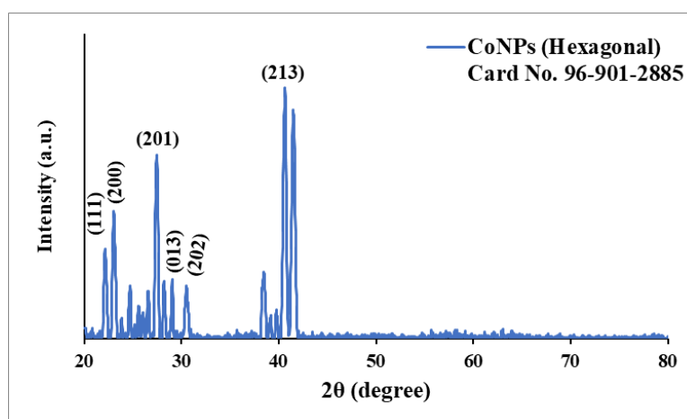
Fig. 2: XRD pattern of CoNPs synthesized physically
