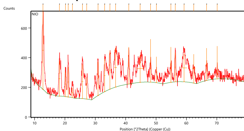
Fig. 3: X-ray diffraction (XRD) pattern of the NiO nanoparticle specimen prepared applying peppermint extract, recorded using Cu K \alpha radiation ( \lambda = 1.5406 \text{ \AA} ), showing the primary peaks corresponding to the (111), (200), and (220) crystal planes
