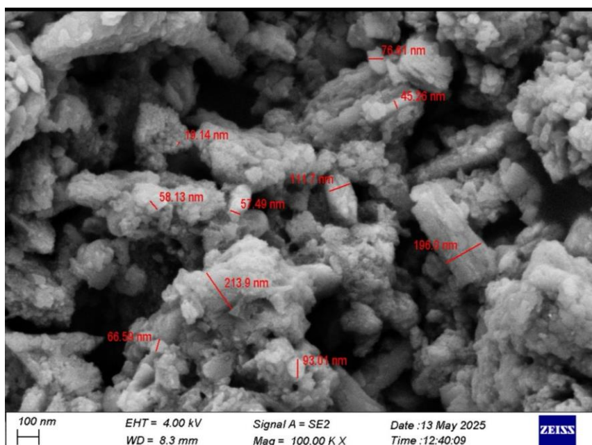
Fig. 4: The SEM micrograph of NiO nanoparticles synthesized using peppermint extract illustrates irregularly formed agglomerates with distinctly porous morphology. The particles demonstrate a size distribution varying from approximately 45 to 213 nm, thereby validating the successful fabrication of nanostructures with heterogeneous dimensional characteristics.
