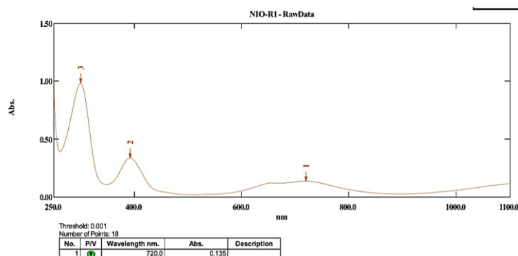
Fig. 1: The UV-Vis absorption spectrum of the nickel oxide nanoparticles synthesized using peppermint extract was recorded in the wavelength range of 250-1100 nm
